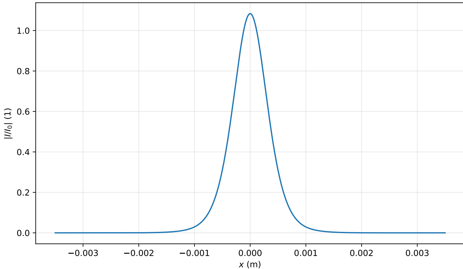
Intensity profile I(x, y = 0, z = 2.070m)/I_0 , P_{in}=0.7P_{cr} , artificial time
